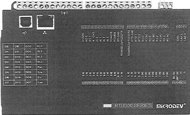
Fotoğraf 3. RTU301-E1N-GA7-B6000 (MODBUS, MQTT, IEC 62056-21, DLMS/COSEM, IEC 60870-5-104, 1 ETH, 2 RS485, 16 DI, 8 DO, 4 AI
